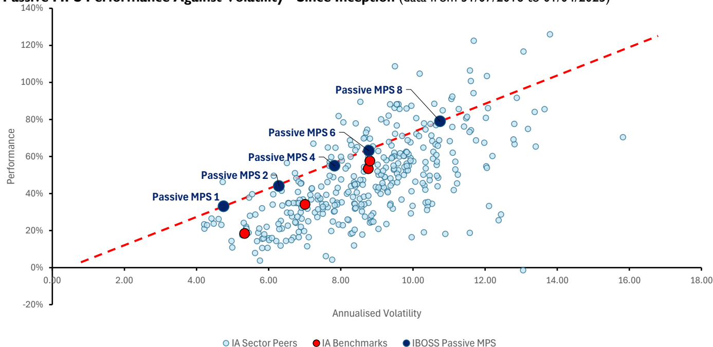
Passive MPS Performance Against Volatility - Since Inception (data from 31/07/2016 to 01/04/2025)
