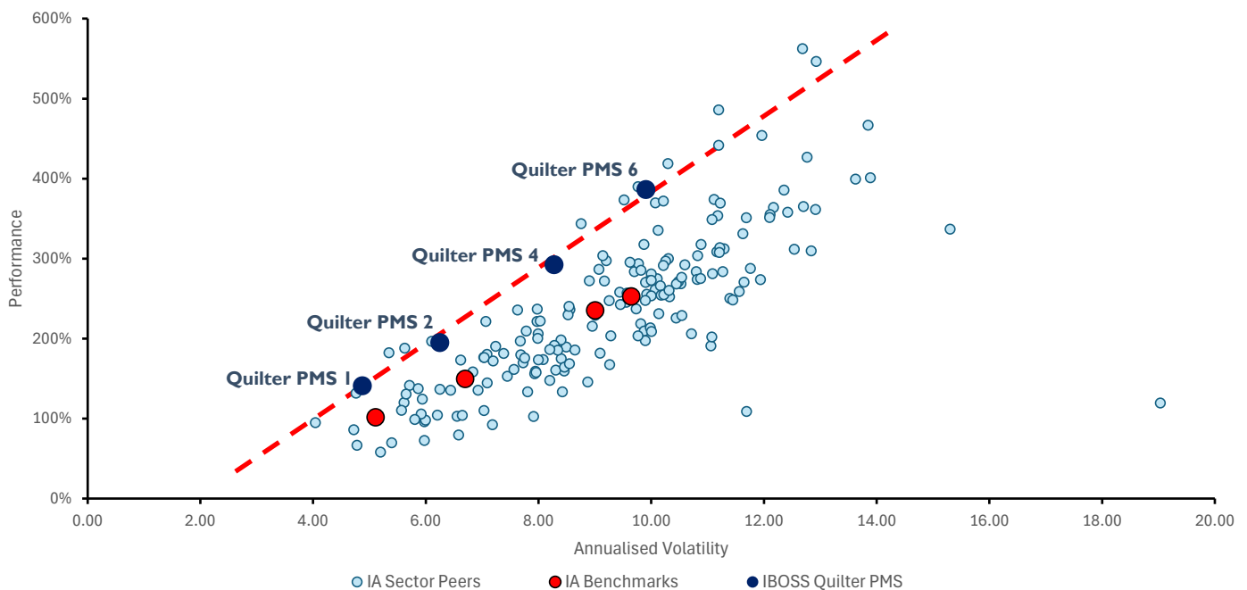
Quilter PMS Performance against Volatility - Since Inception (data from 31/10/2008 to 31/03/2026)
