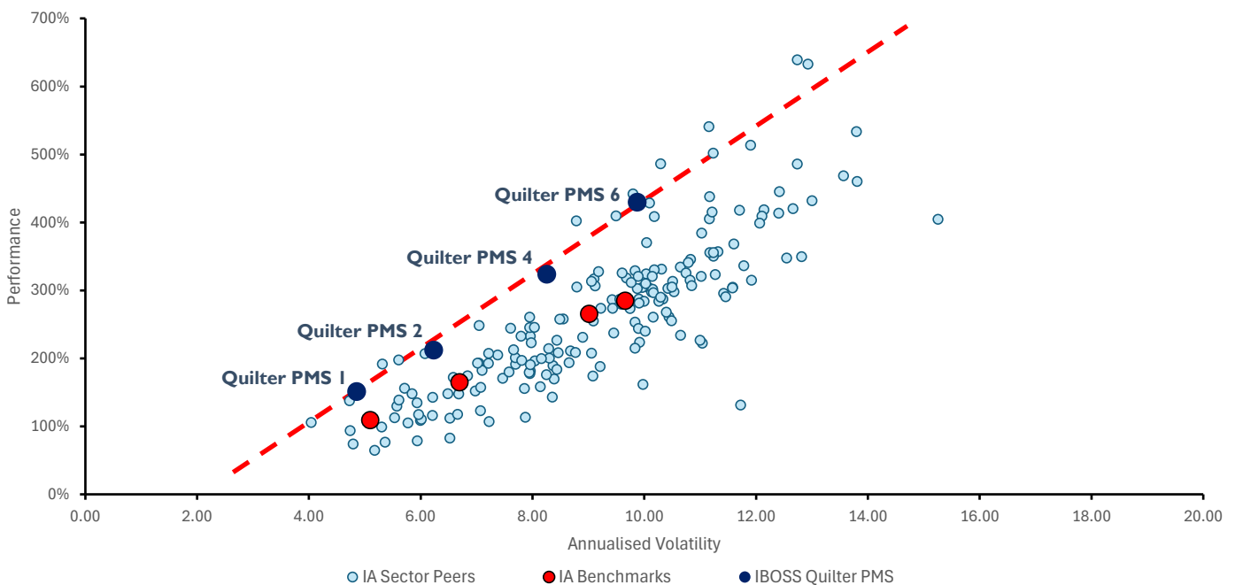
Quilter PMS Performance against Volatility - Since Inception (data from 31/10/2008 to 31/07/2026)
